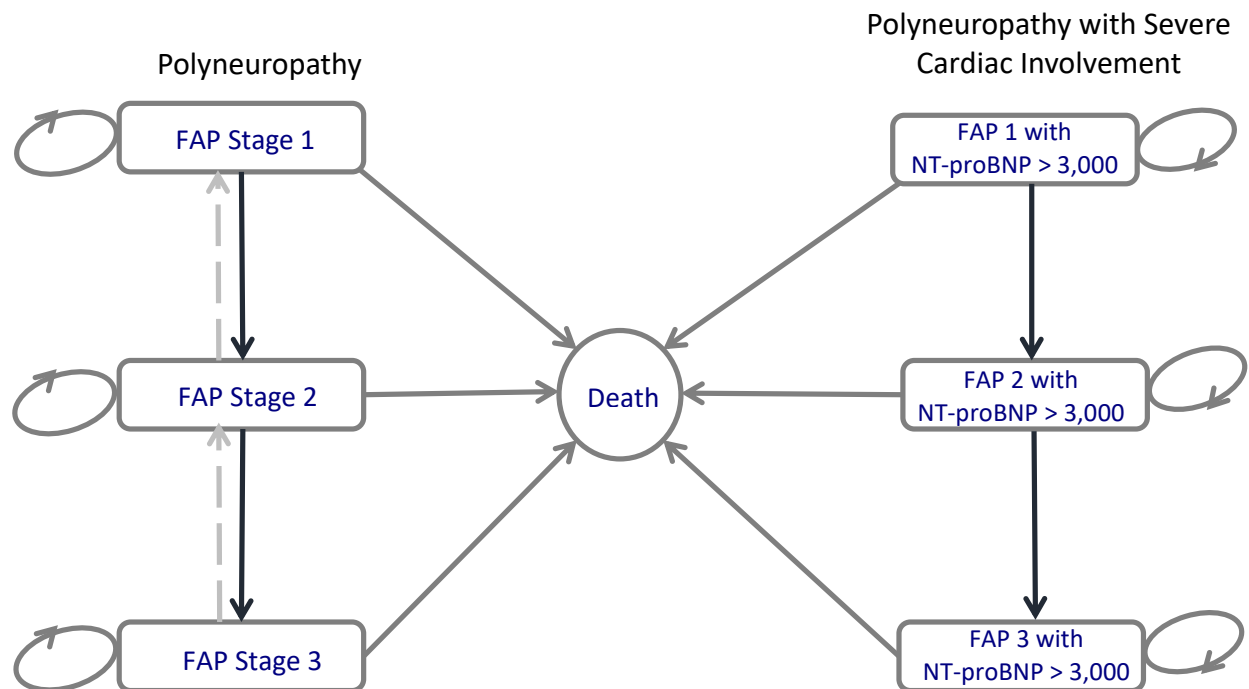
Figure 4.1. Model Framework
