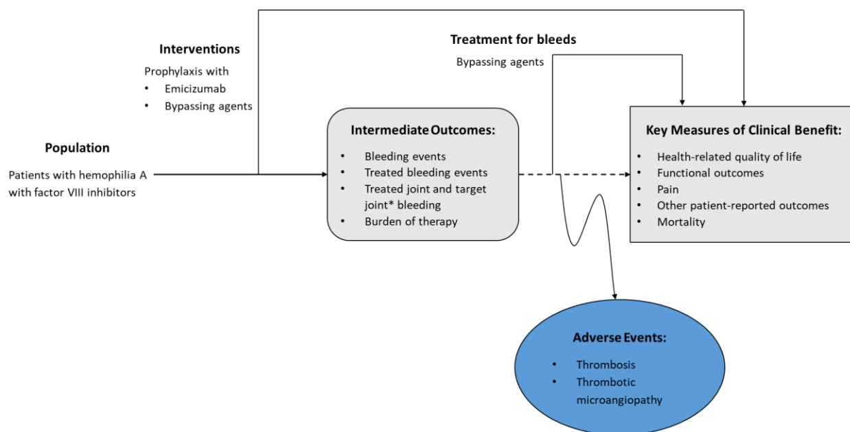
Figure 1.2. Analytic Framework
