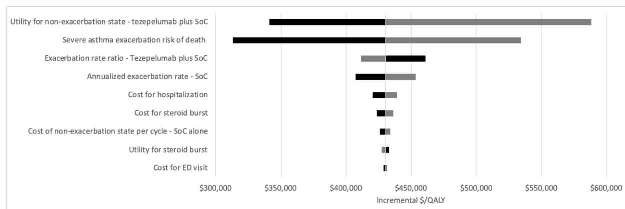
Figure 4.2. Tornado Diagram
