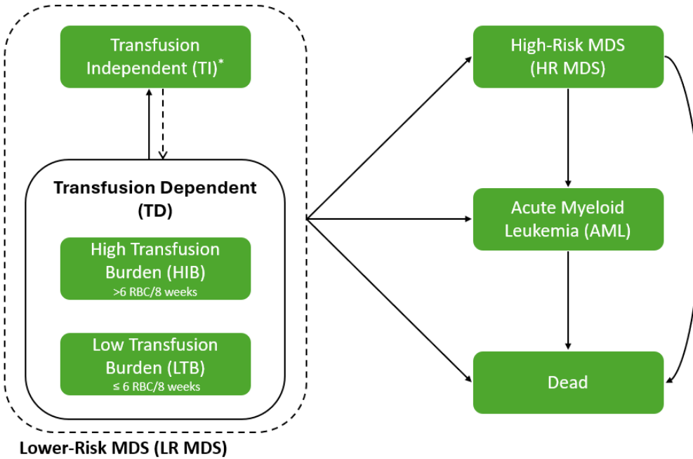
Figure 4.1. Model Structure
