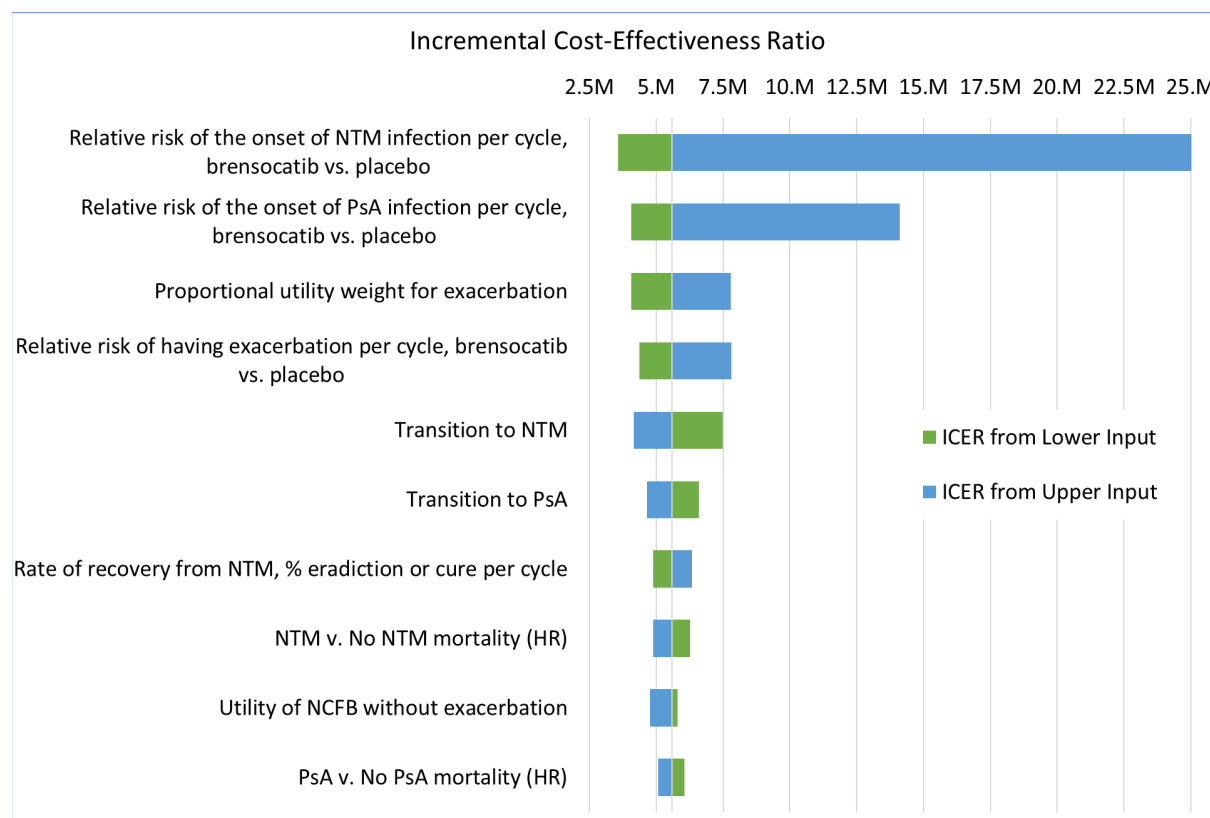
Figure 4.2. Tornado Diagram
