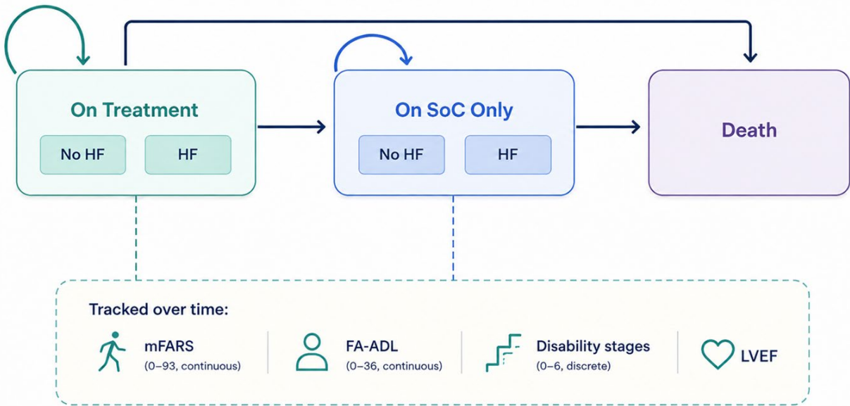
Figure 4.1. Model Structure
